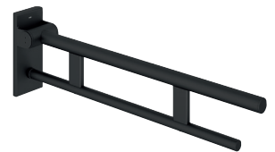
Stützklappgriff Duo Design A 900.50.10160 | 600 mm 900.50.10260 | 700 mm Stützklappgriff Duo mobil 900.50.40160 | 600 mm 900.50.40260 | 700 mm
